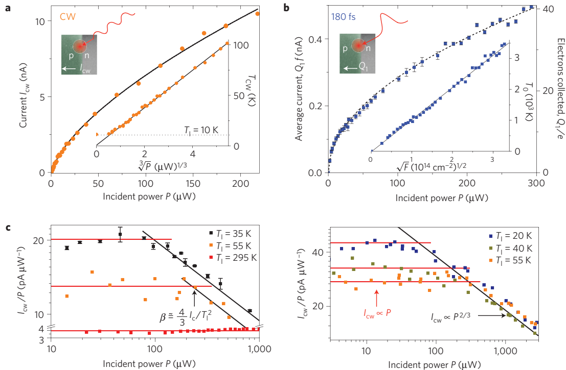
Figure 3 | PC response obeys SC power laws. a , PC generated under CW excitation at a graphene p–n junction scales as P^{0.65 \pm 0.02} (black line). Inset: Corresponding electron temperatures scale linearly with \sqrt[3]{P} . b , PC ( Q_1 f ) and corresponding number of electrons collected per pulse ( Q_1/e ) versus pulsed laser power. The dashed black line indicates the power law fit of P^{0.50 \pm 0.03} . Inset: Same plot showing the corresponding initial temperatures ( T_0 ) versus photon fluence (square root scale). c , The CW power PC dependence changes from linear (red lines) to a P^{2/3} power (black lines) at an increasing cross-over current, I_c as T_1 is raised. From I_c we calculate \beta for our experimental conditions (left panel) and a different CVD device (right panel).
