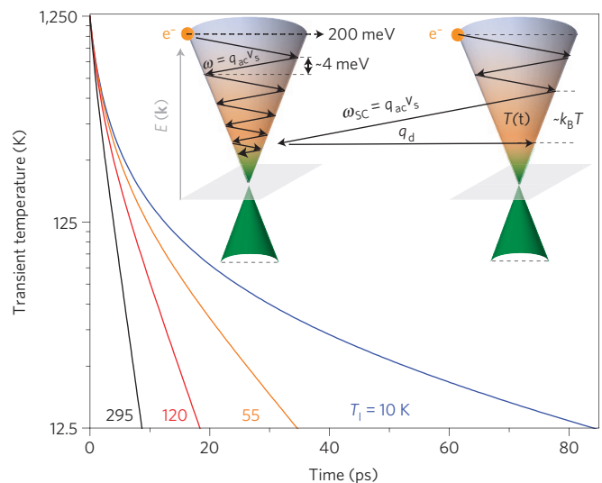
Figure 1 | Hot-electron cooling by acoustic phonons. Solving the SC rate law dT/dt = -(A/\alpha)(T^3 - T_1^3)/T , we plot the predicted cooling of the graphene hot-electron temperature T(t, T_1) - T_1 (logscale). The thermal decay changes from inverse to exponential with increasing lattice temperature. Left inset: Momentum conservation restricts cooling of hot carriers ( e^- ) near the Fermi level (green) to low energy ( \lesssim 4 meV) acoustic phonon emission (black arrows, scale exaggerated, q_{ac} is the acoustic phonon wavevector). Right inset: In a SC transition the momentum restrictions is relaxed by the lattice disorder ( q_d ), enabling faster cooling by emission of high-energy ( \sim k_B T ) acoustic phonons.
