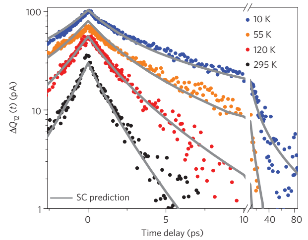
Figure 5 | SC model predicts TPC dependence on T_1 . At constant incident power, the TPC response varies considerably on warming to 295 K. Using the SC temperature response in Fig. 1, we calculate the predicted TPC response \Delta Q_{12}(t_d) with no free parameters (grey lines).
