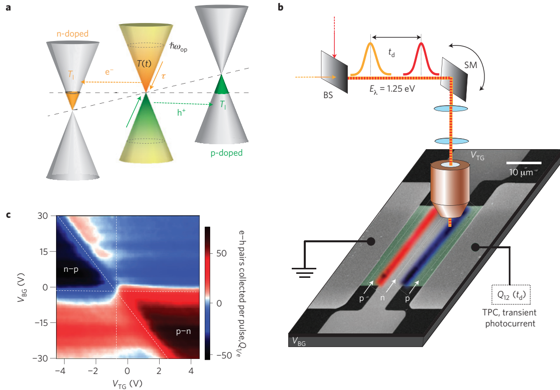
Figure 2 | Photocurrent set-up, a time-resolved graphene thermometer. a , The temperature T(t) of thermalized hot electrons ( e^- ) and holes ( h^+ ) in a graphene p-n junction cool at a characteristic rate \tau^{-1} . The elevated junction temperature drives the collected thermoelectric current. b , Experimental set-up where we collect PC from graphene as a function of T_1 , laser power and two-pulse time delay ( t_d ). Graphene (green, false colour) is excited using a focused CW or pulse laser via a piezo scanning mirror (SM). The device SEM shows an overlay of a spatial PC map with peaks for the graphene p-n (0.7 nA, red) and n-p junctions (−0.6 nA, blue). BS, beamsplitter. c , Pulsed excitation PC map, plotting electrons collected ( Q_1/e ) versus applied gate voltages. Tuning the electrostatic gates ( V_{TG} and V_{BG} ) show six PC regions (dotted lines).
