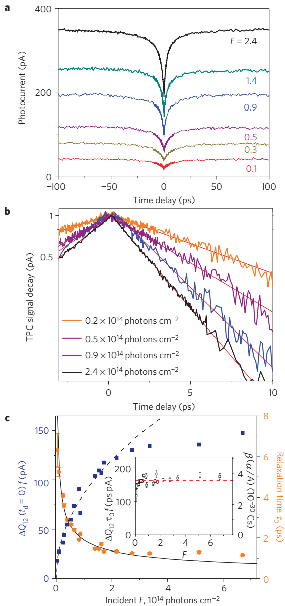
Figure 4 | Extracting the hot-electron relaxation time. a , Collected two-pulse photocurrent ( Q_{12}(t_d)f ) response at selected incident photon fluences (in units of \times 10^{14} photons \text{cm}^{-2} ). b , As shown, the decay of the TPC signal ( \Delta Q_{12}(t_d)f , normalized) is closely linearized when plotted on an inverse scale. c , TPC peak amplitude (square root fit, dashed line) and \tau_0 (inverse root fit, black line) versus laser fluence, F . Inset: The product of the data points yields a constant \Delta Q_{12}(0)f\tau_0 = 160 \pm 13 ps pA (dashed red line) or an electron cooling rate of A/\alpha of \sim 5.5 \times 10^8 \text{ K}^{-1} \text{ s}^{-1} .
